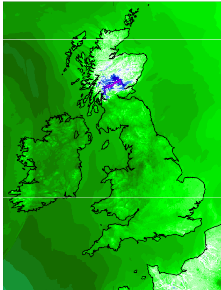
UKV op Temperature at 1.5m [C] Monday 0300Z 22/03/2010 (+0h)
